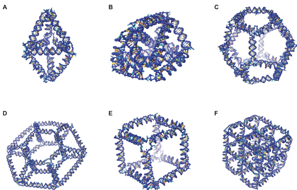
Figure 2. oxDNA models of Sterna designs for RNA meshes. (A) Bipyramid. (B) Prism (sides triangulated). (C) Dodecahedron. (D) Toroid. (E) Cube. (F) 2x2x2 Cube.
